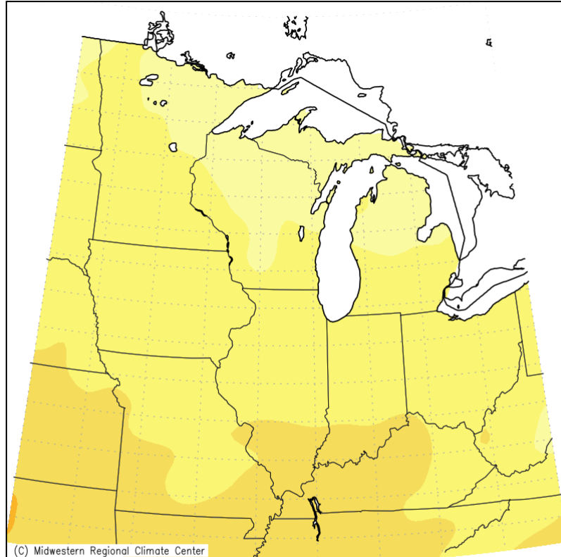
Average Temperature (°F) September 1, 2024 to September 30, 2024
