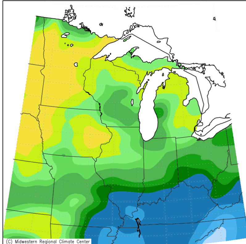
Accumulated Precipitation (in) September 1, 2024 to September 30, 2024
