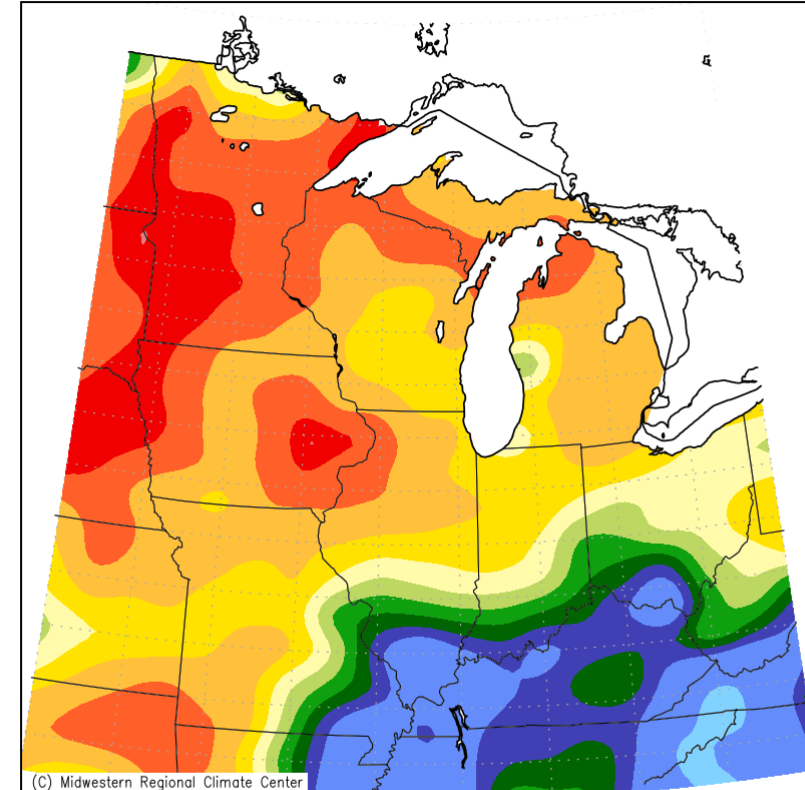
Accumulated Precipitation: Percent of Mean September 1, 2024 to September 30, 2024
