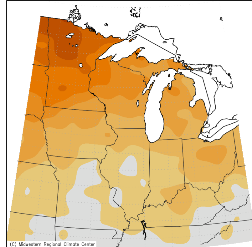
Average Temperature (°F): Departure from Mean September 1, 2024 to September 30, 2024
